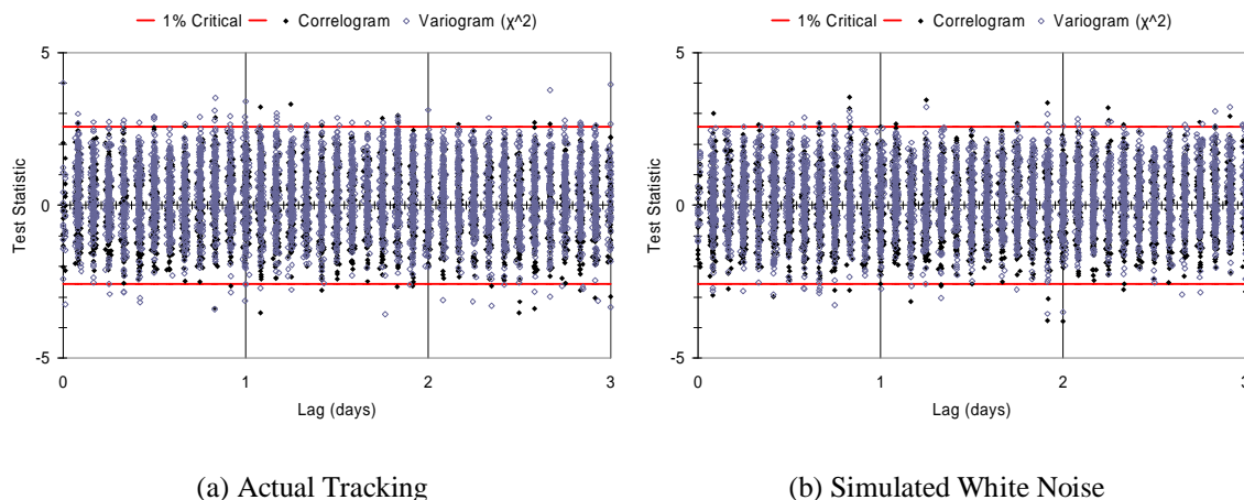
Figure 2. Correlation Test Statistics for Sample Tracking Tested at 1% Significance.
