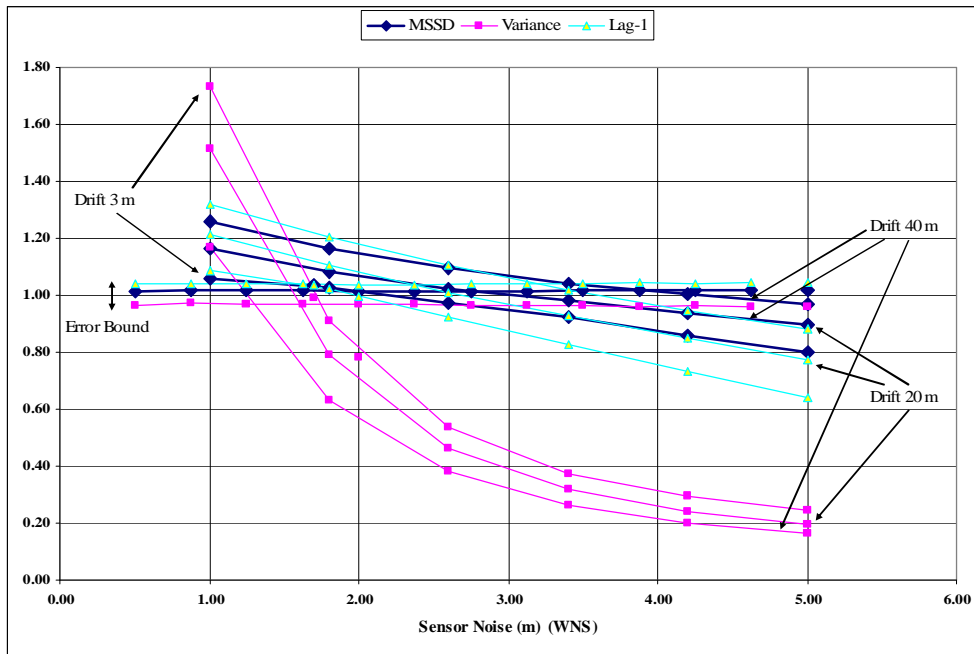
Figure 4. Tracker Parameter Trends.
