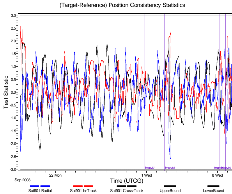
Figure 7. Filter Smoother Position Consistency Test.
