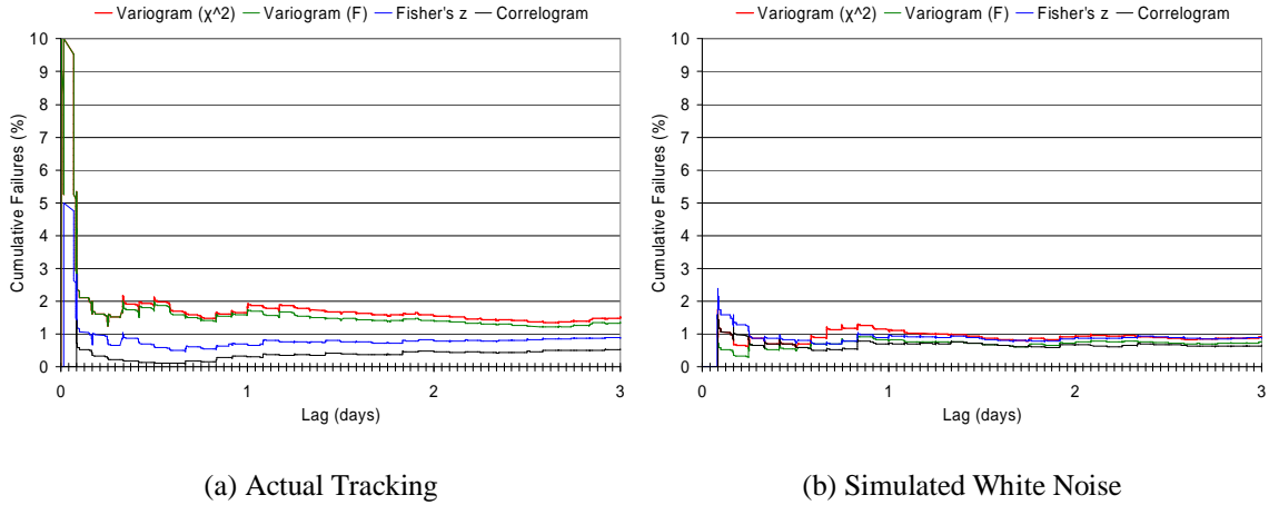
Figure 3. Cumulative False Alarms for Sample Tracking Tested at 1% Significance.
