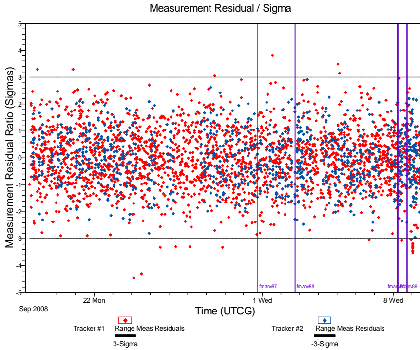
Figure 6. Tracking-Station Residual Ratios.
